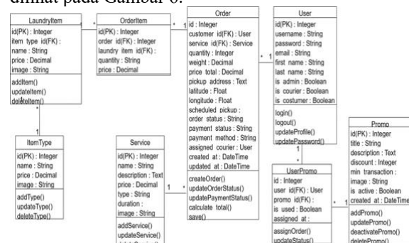
Gambar 6. Class Diagram
